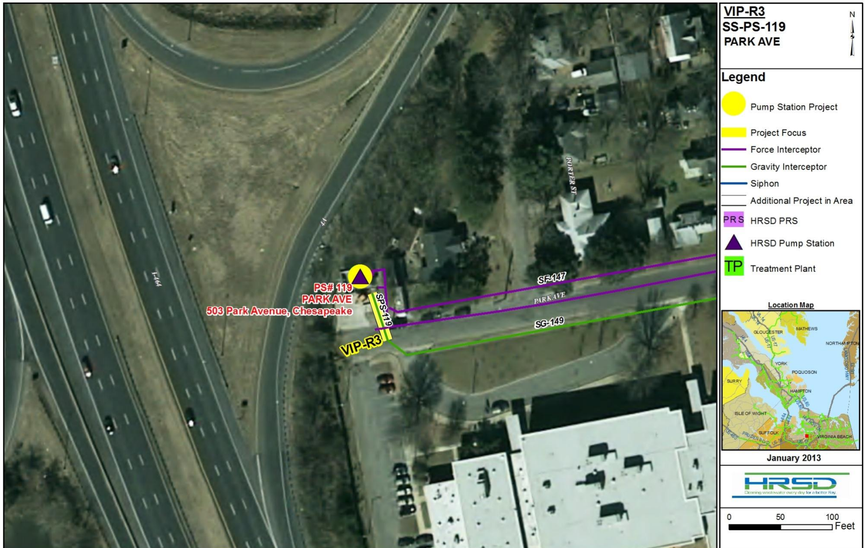
Figure 4-66. Project VIP-R3. Sheet 1 of 1.
