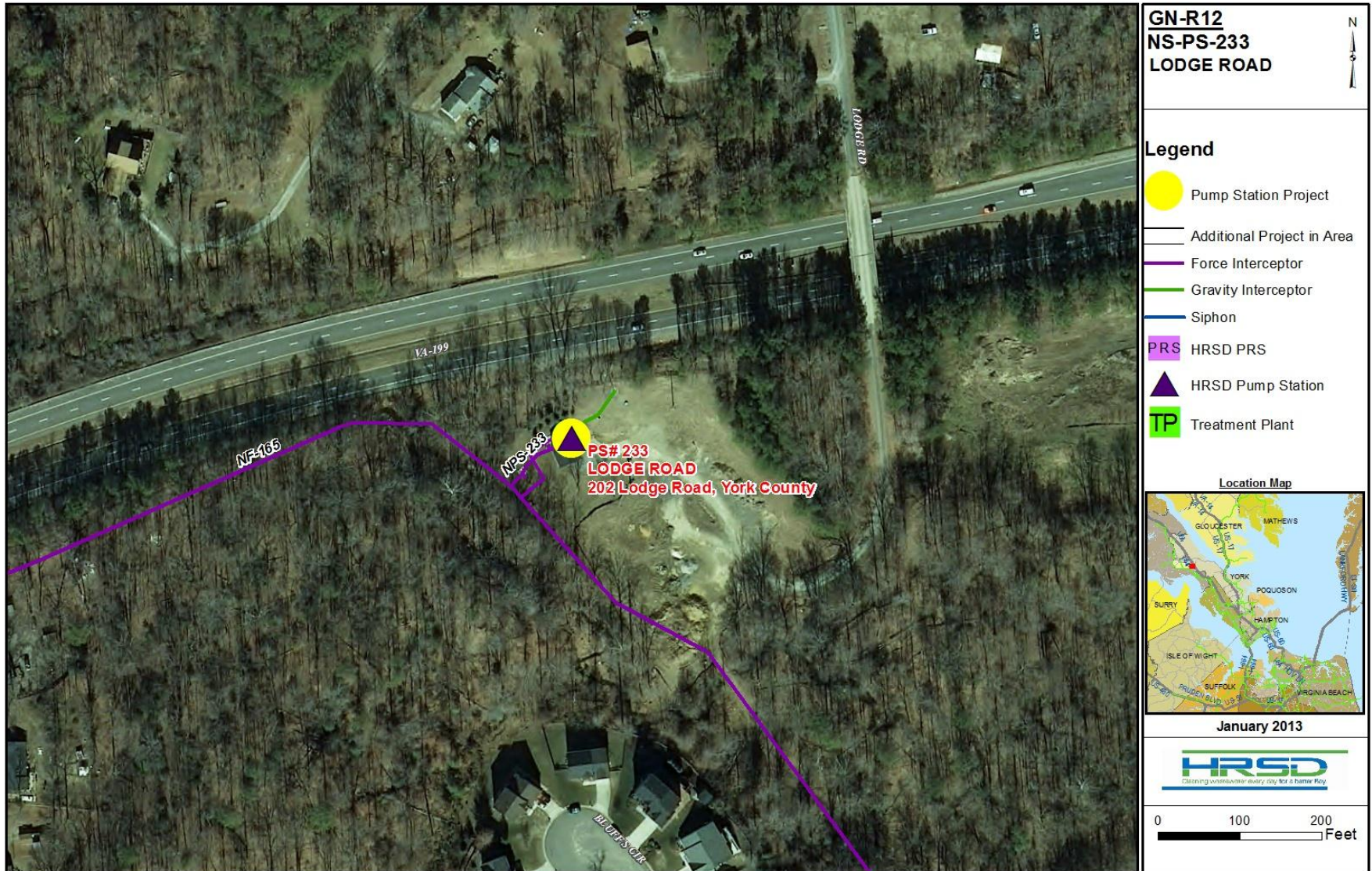
Figure 4-57. Project GN-R12. Lodge Road. Sheet 3 of 3.
