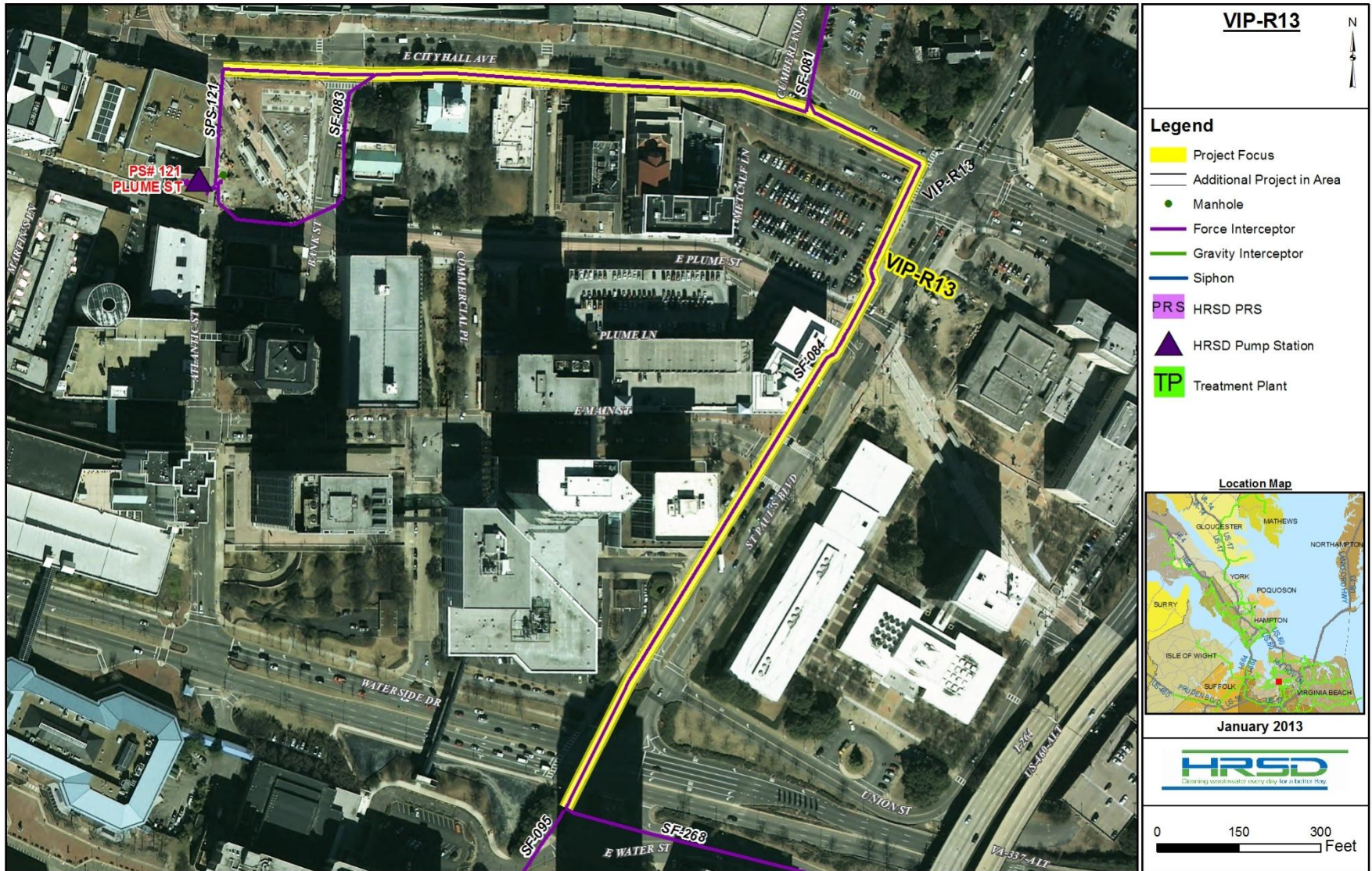
Figure 4-82. Project VIP-R13. Sheet 1 of 1.
