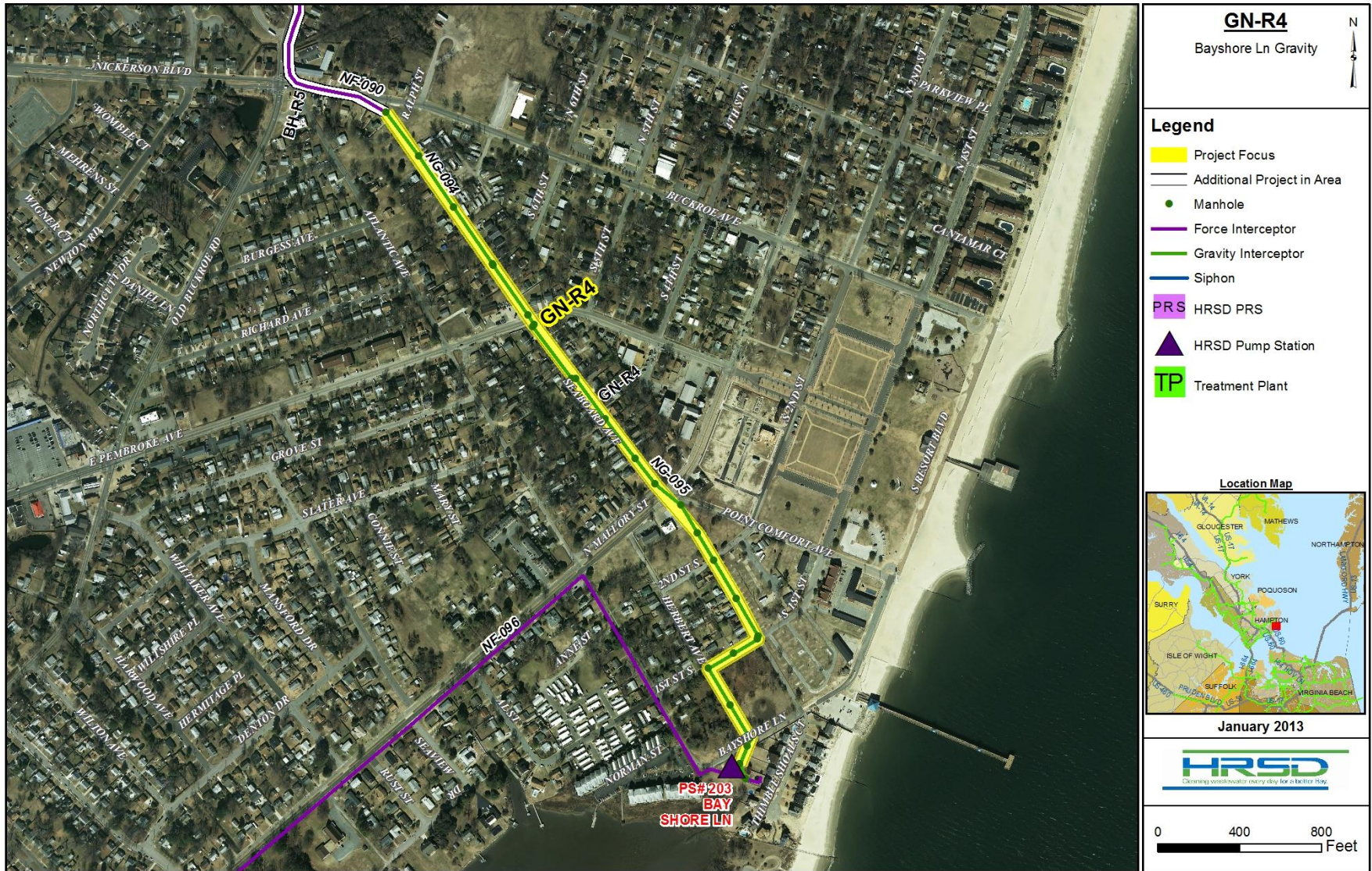
Figure 4-41. Project GN-R4. Bayshore Ln. Sheet 3 of 8.
