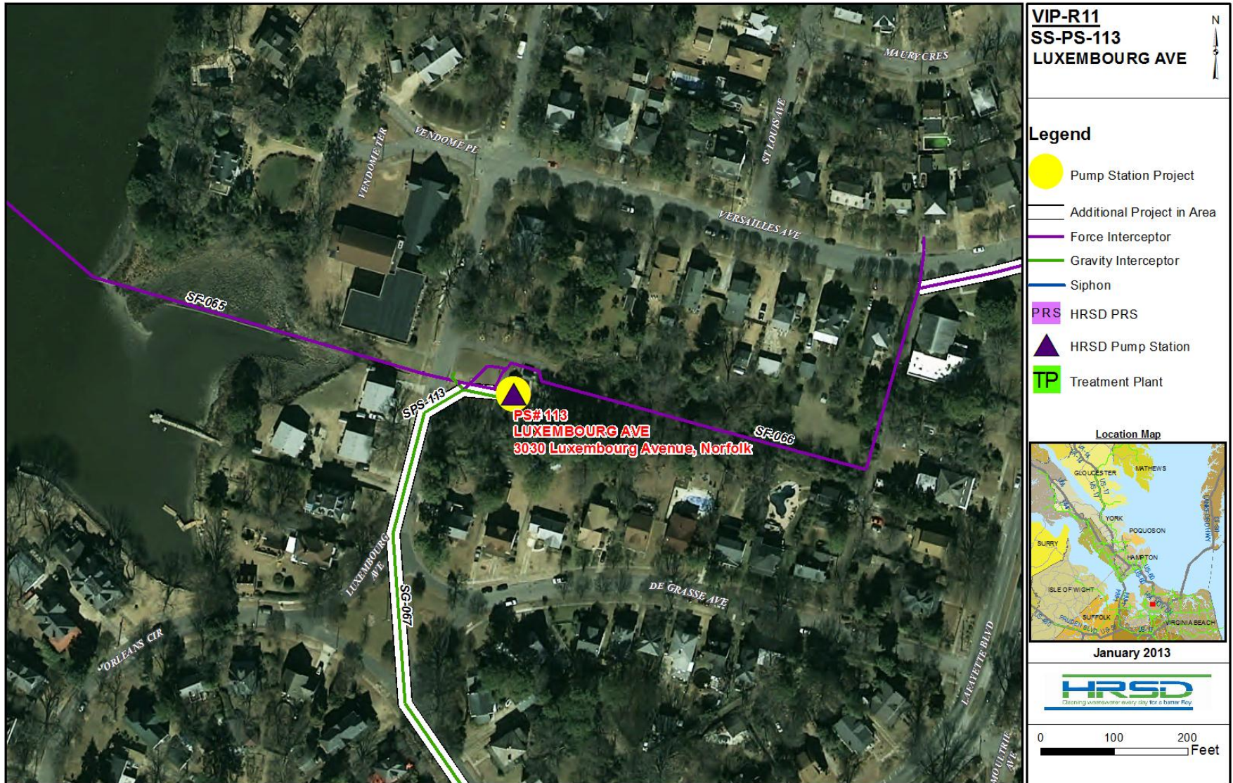
Figure 4-79. Project VIP-R11. Luxemburg Ave. Sheet 3 of 4.
