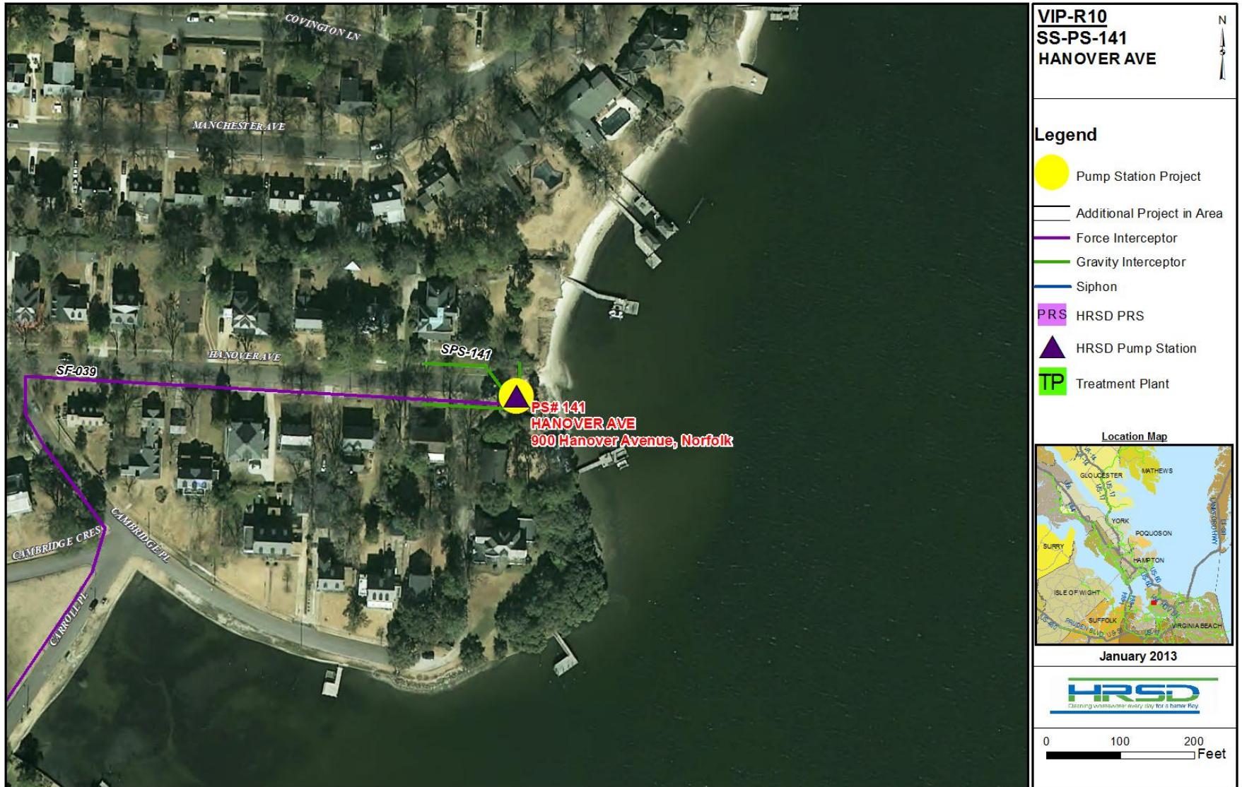
Figure 4-73. Project VIP-R10. Hanover Ave. Sheet 2 of 5.
