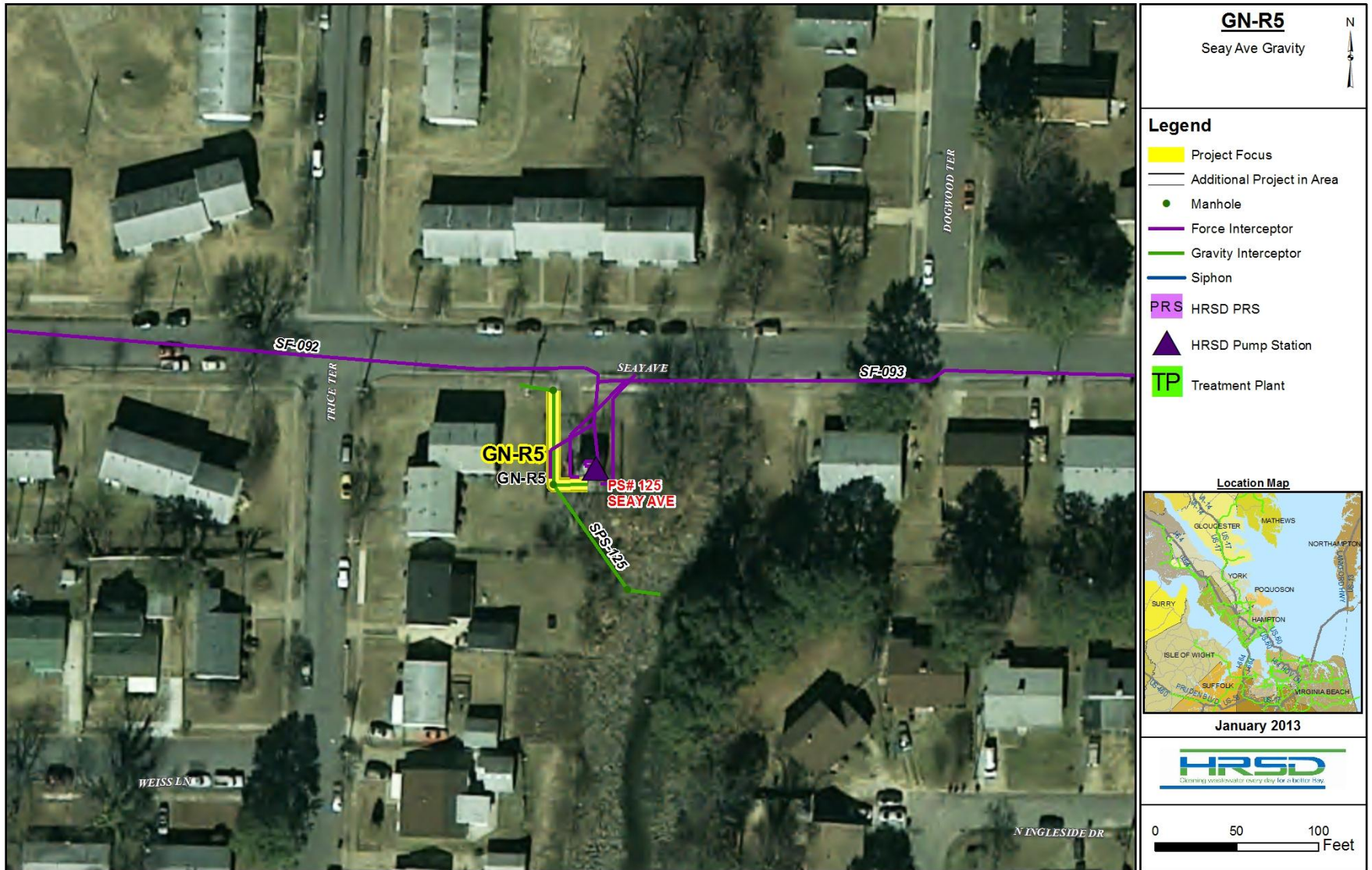
Figure 4-50. Project GN-R5. Seay Ave. Sheet 4 of 6.
