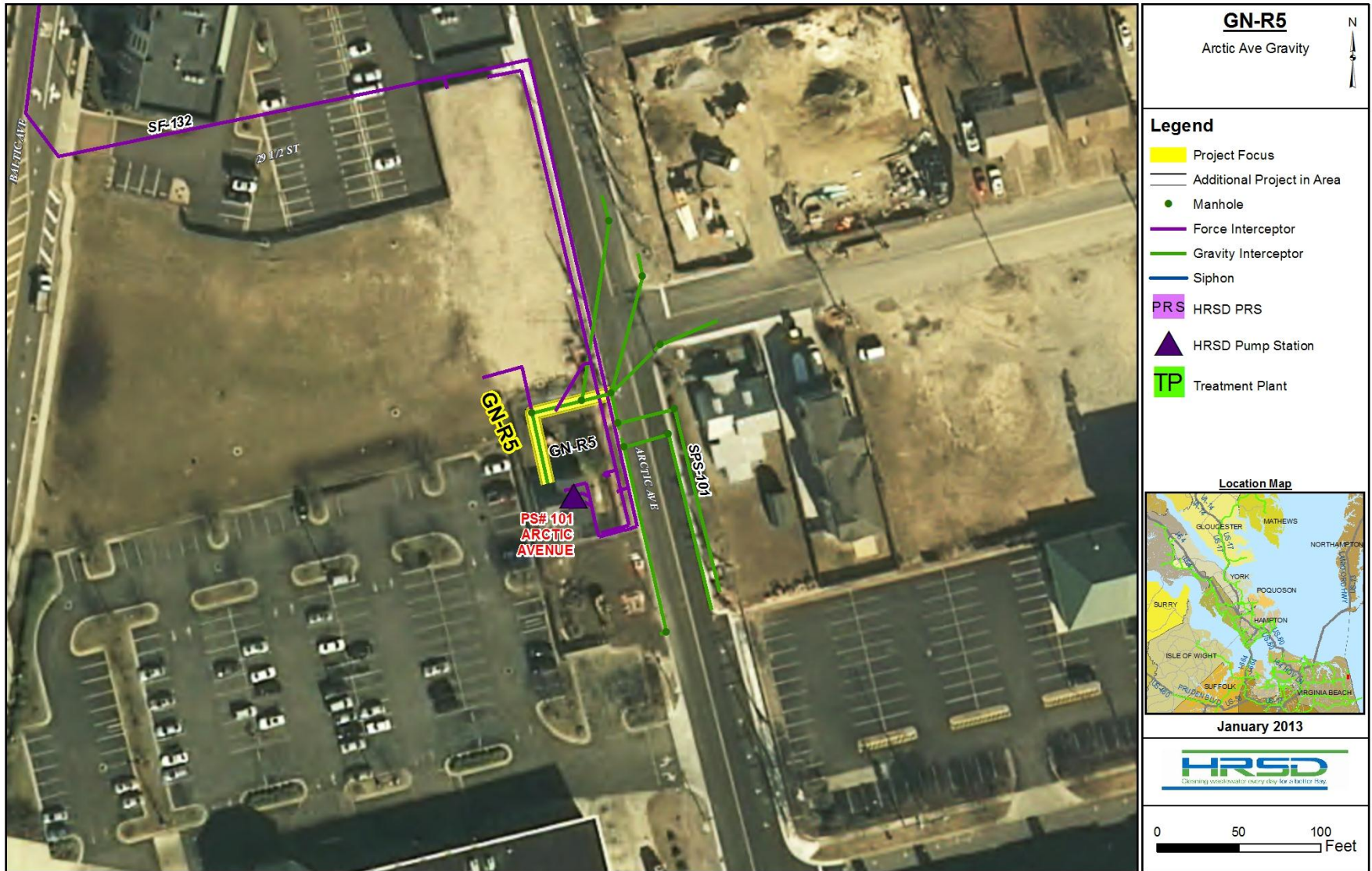
Figure 4-49. Project GN-R5. Arctic Ave. Sheet 3 of 6.
