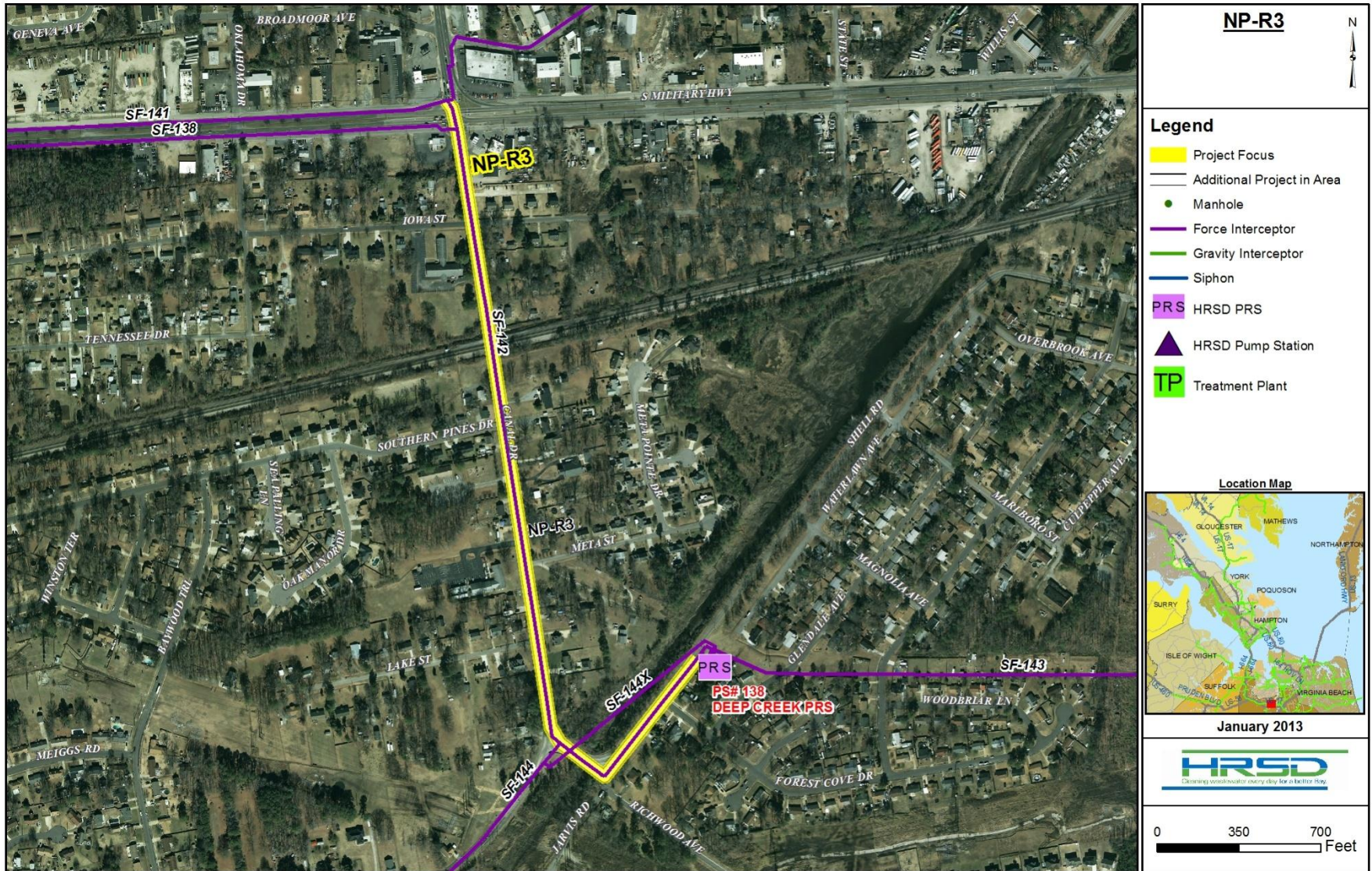
Figure 4-62. Project NP-R3. Sheet 1 of 1.
