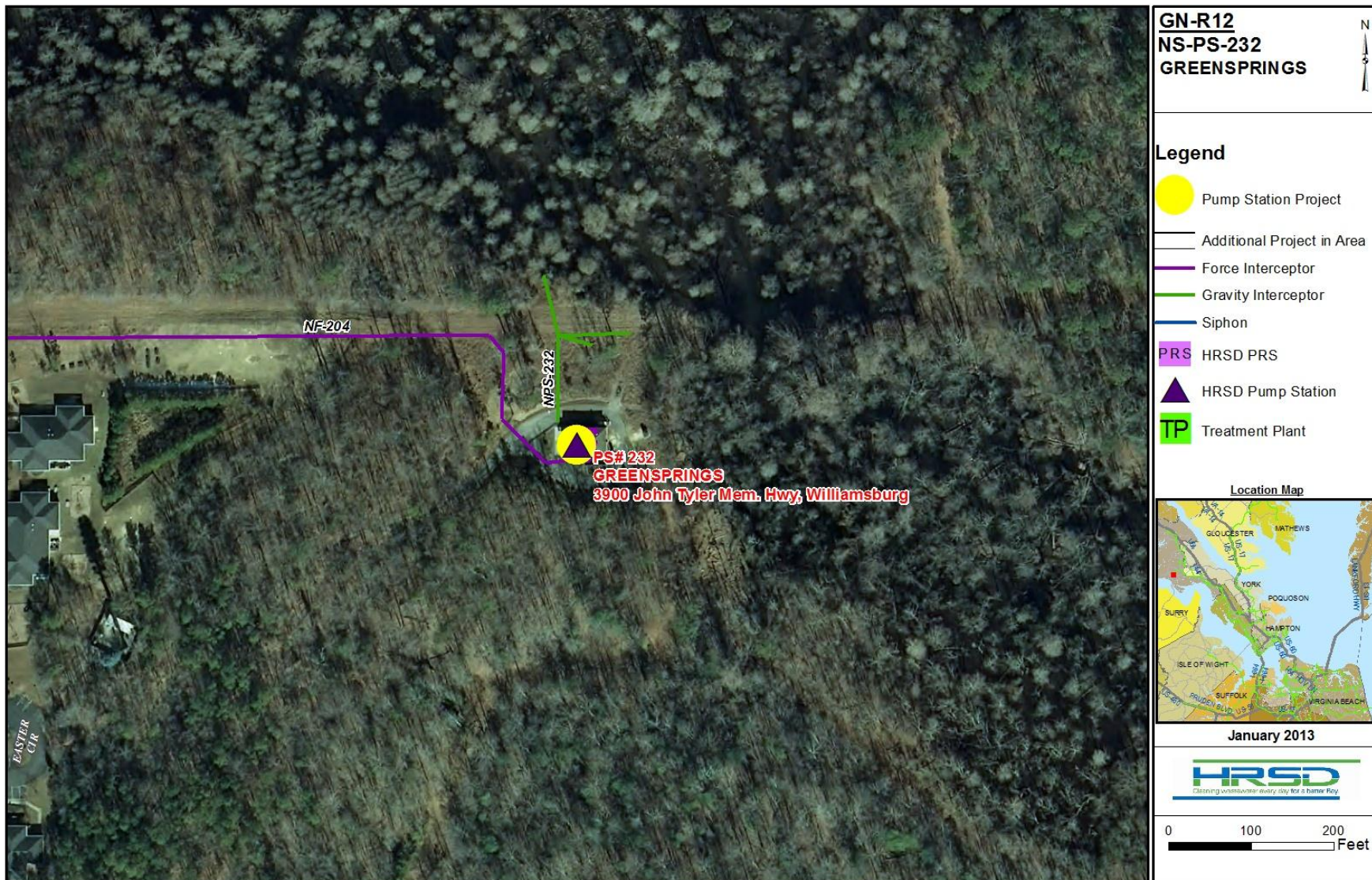
Figure 4-56. Project GN-R12. Greensprings. Sheet 2 of 3.
