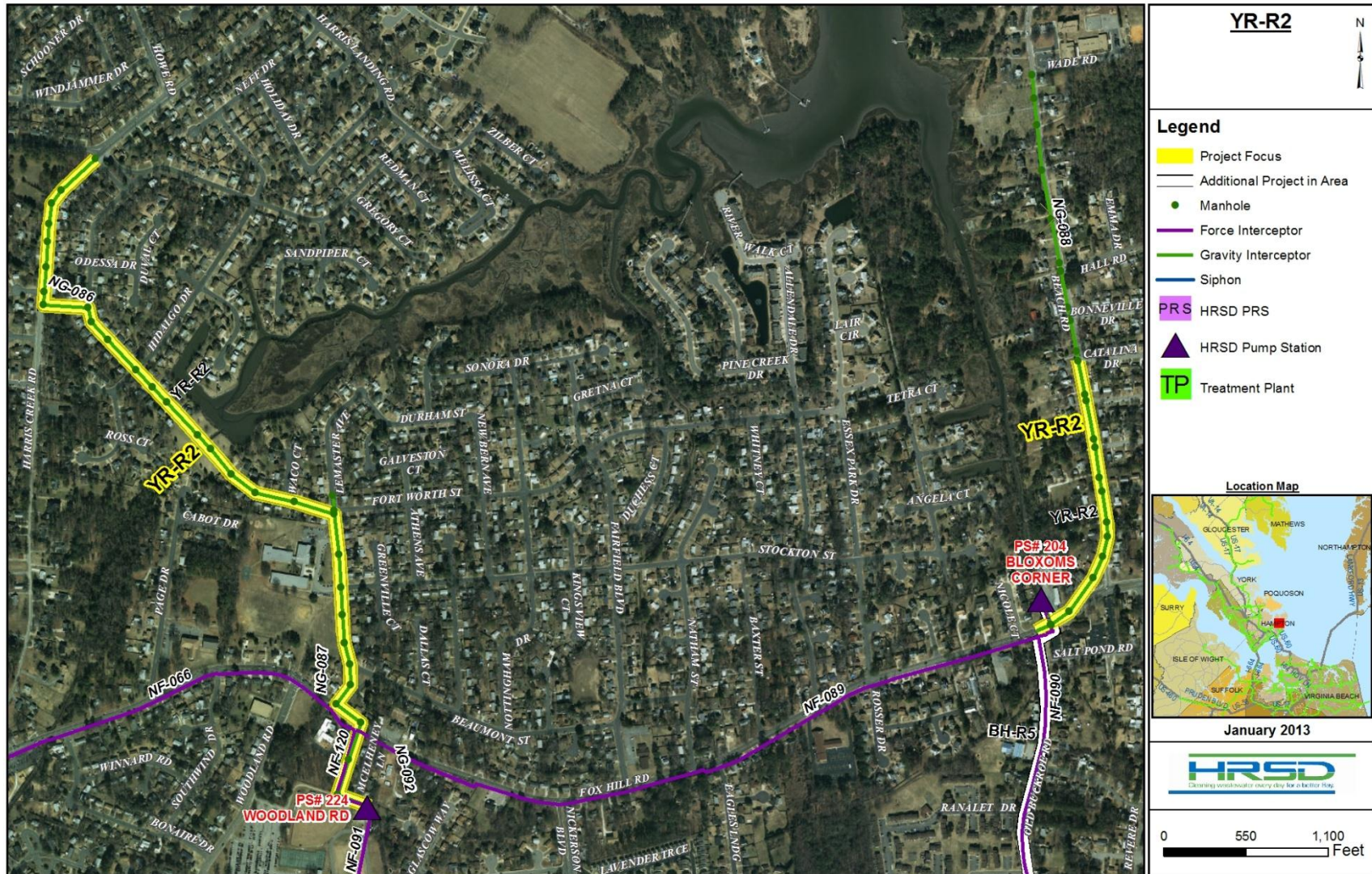
Figure 4-87. Project YR-R2. Sheet 1 of 1.
