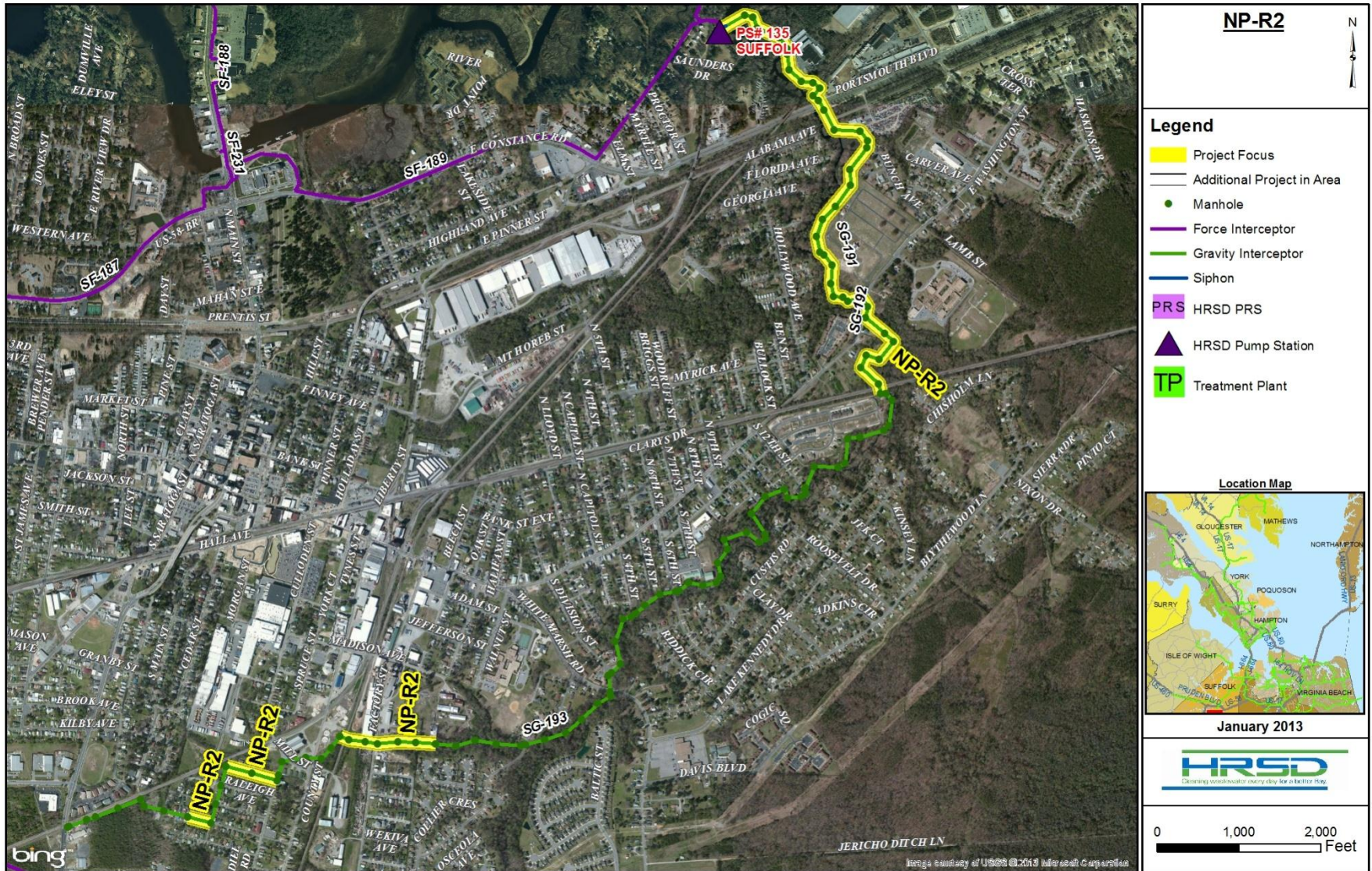
Figure 4-61. Project NP-R2. Sheet 1 of 1.
