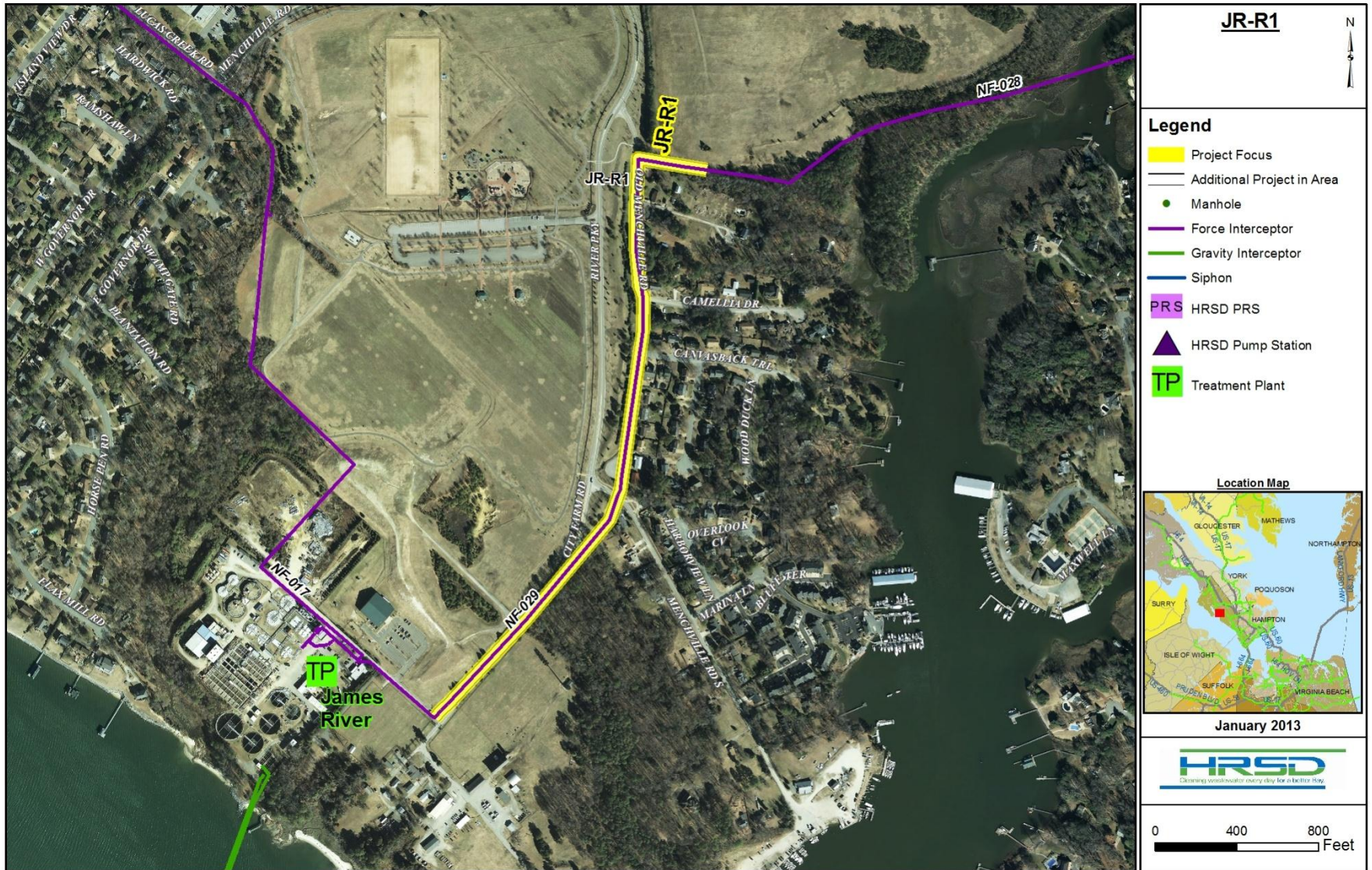
Figure 4-58. Project JR-R1. Sheet 1 of 1.
