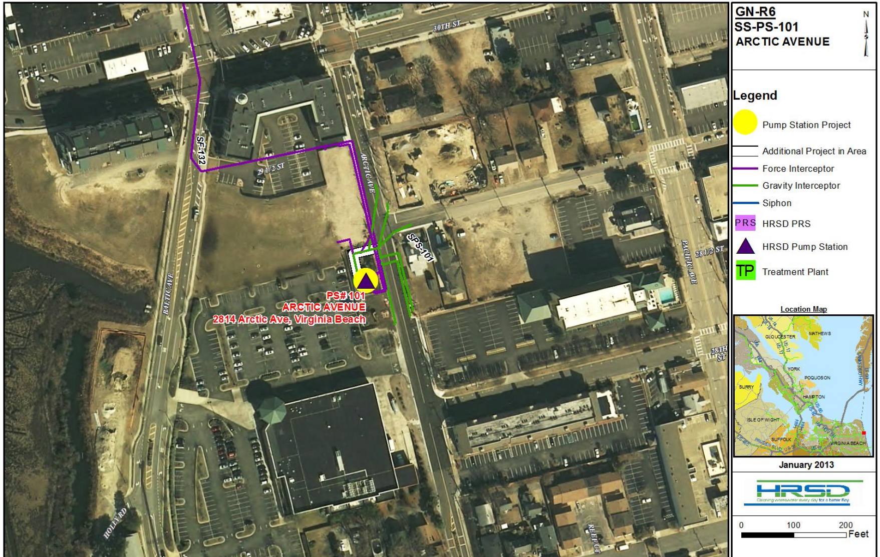
Figure 4-53. Project GN-R6. Arctic Ave. Sheet 1 of 2.
