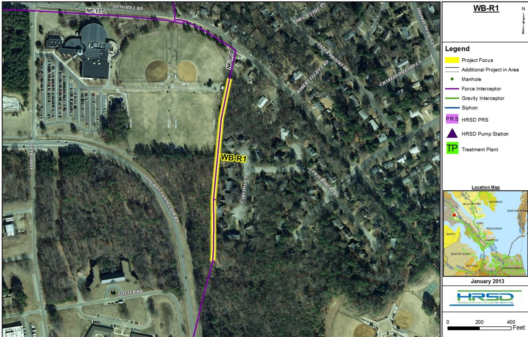
Figure 4-85. Project WB-R1. Sheet 1 of 1.
