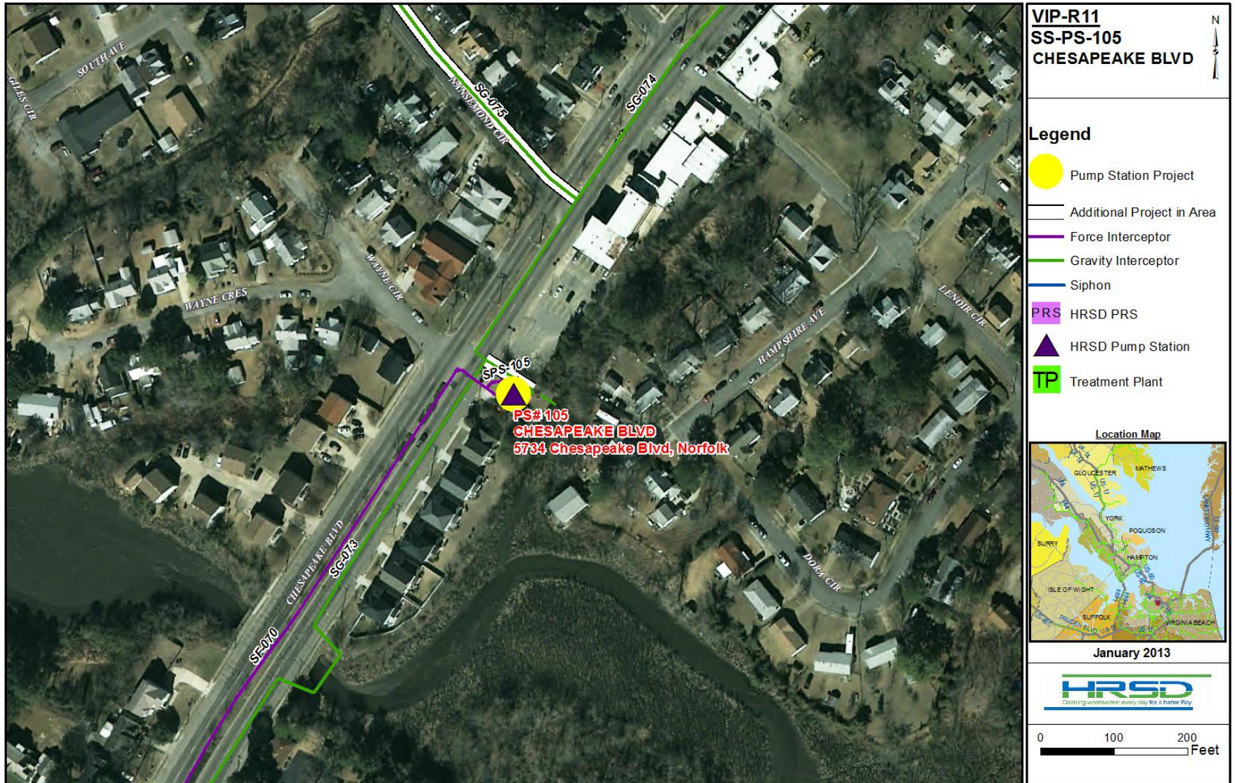
Figure 4-78. Project VIP-R11. Chesapeake Blvd. Sheet 2 of 4.
